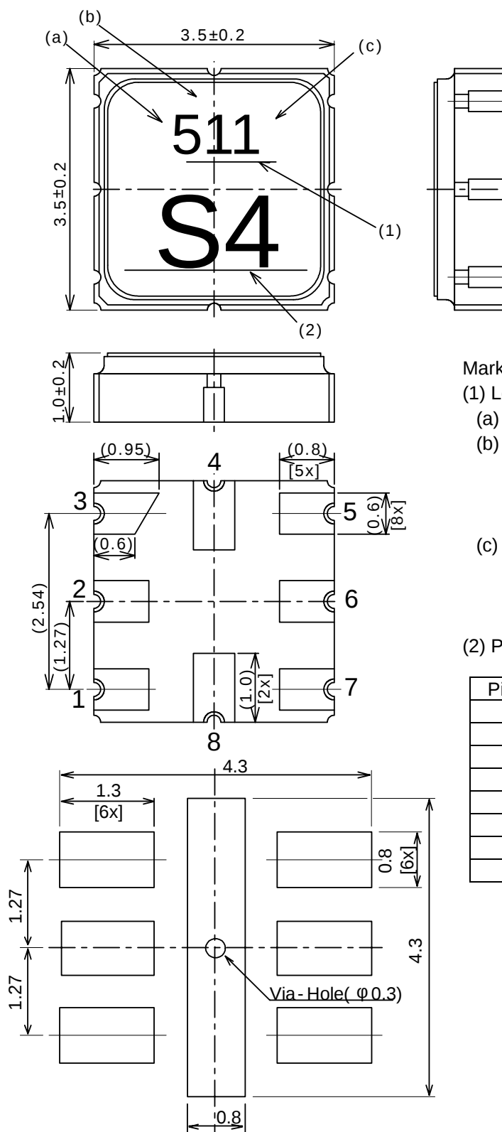
Fig.3 Desirable land area (in mm)
